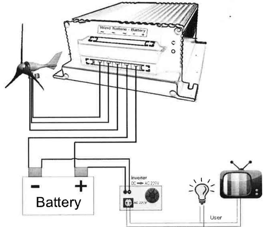
Wiring diagram for an example
